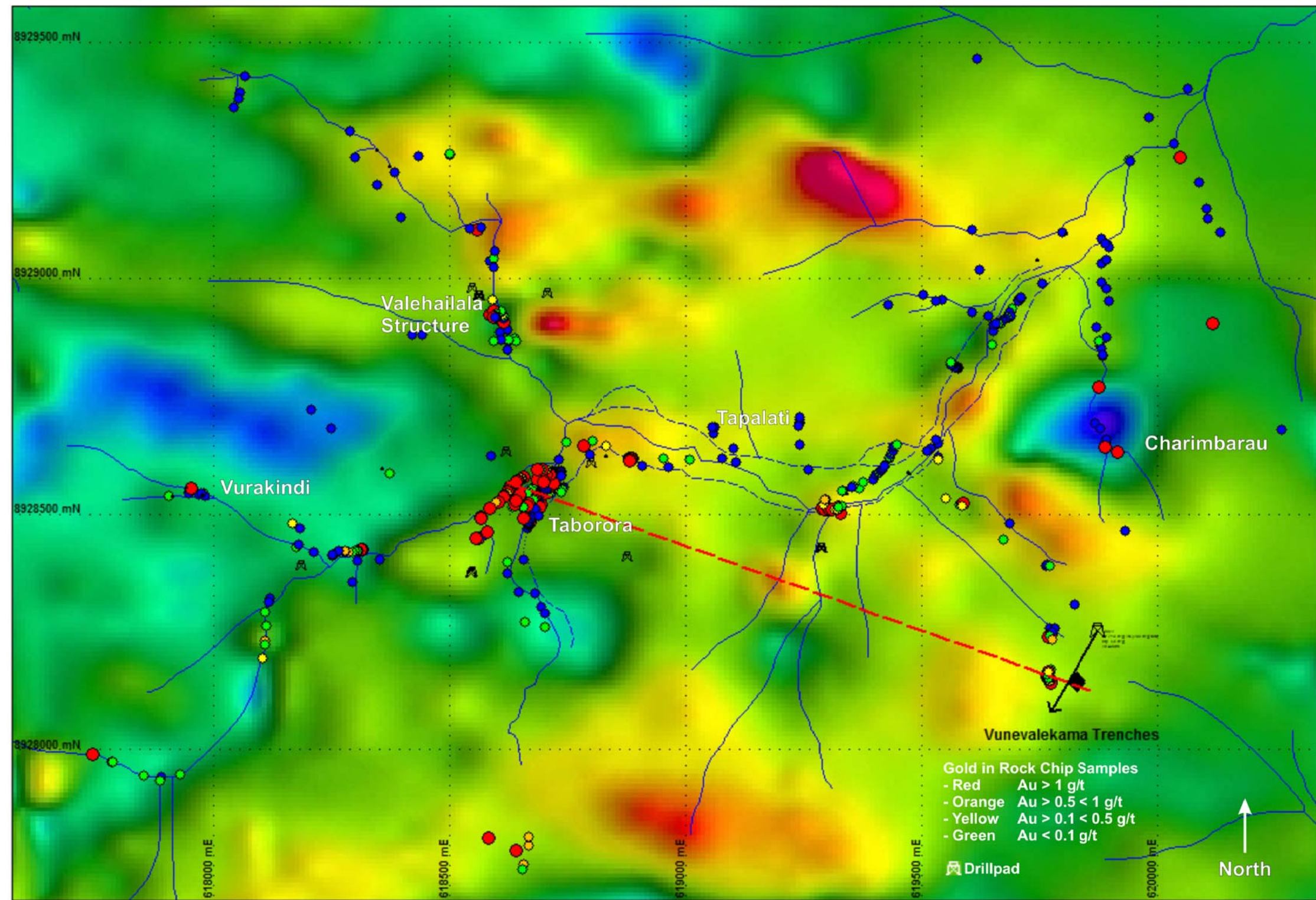
Sutakiki Prospects: rock chip gold values on Aeromagnetic background. May 2008
